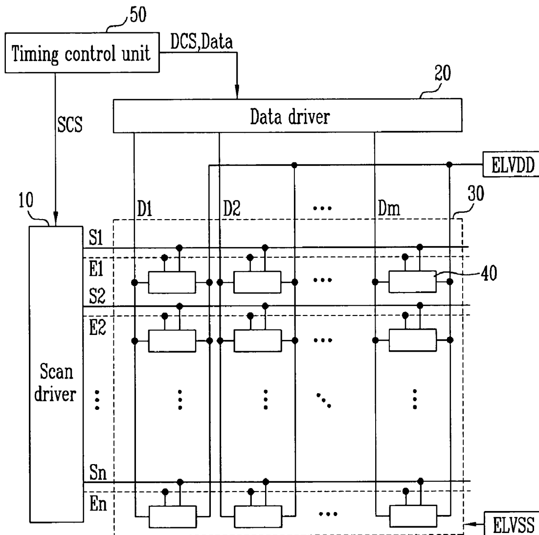
FIG. 1 (PRIOR ART)
